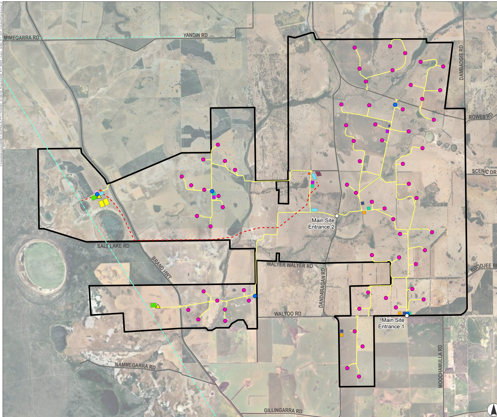
FIGURE 2.1 Indicative Project Layout
