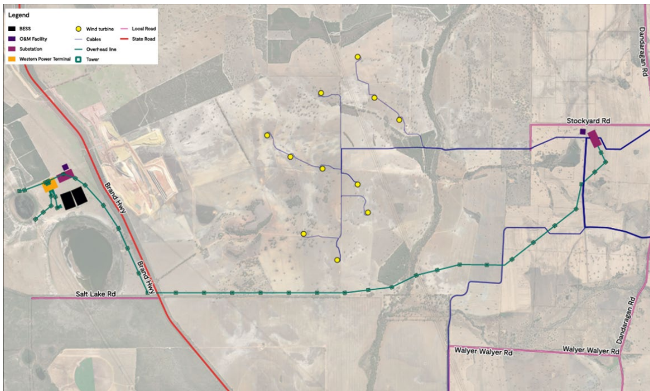
Figure 2.2 Conceptual layout of OHL Transmission route and infrastructure
